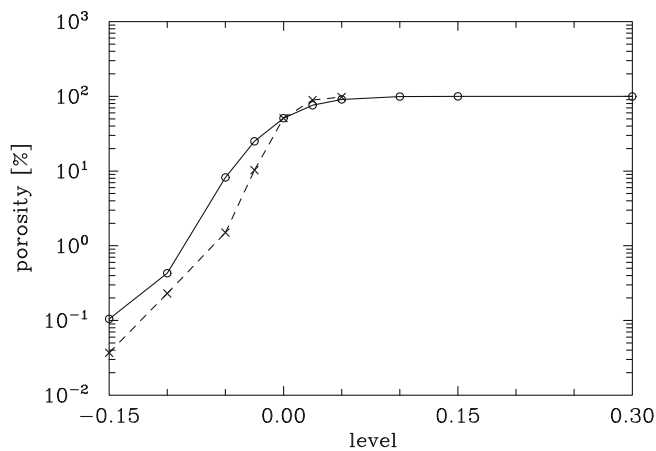
Fig. 11. Porosity in function of \gamma ; circles and crosses correspond to m = 4 and m = 16 filter iterations.
