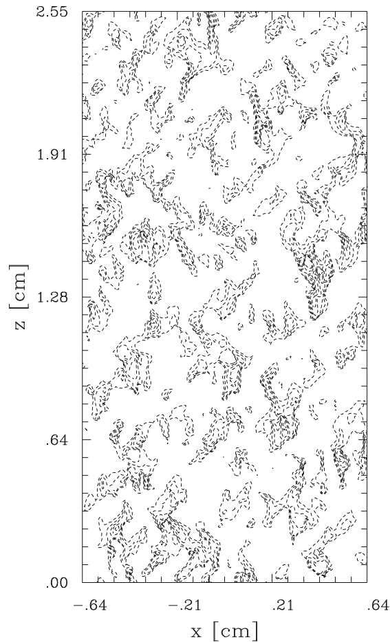
Fig. 6. Instantaneous vertical velocity in the central xz plane at t = t_0 + 5 \cdot 10^{-2} ; contours in the range [-18.75 \cdot 10^{-2}, -\Delta w] \text{ms}^{-1} are shown with the interval \Delta w = 3.125 \cdot 10^{-2} \text{ms}^{-1} .
